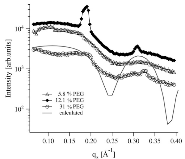
FIGURE 5 Sections along q_z through the pore signal of samples with P/L = 1:12.5 at different osmotic pressures ( symbols ) for q_y = 0.1 \text{ \AA}^{-1} and cut through the square of the simulated form factor |F(q_z)|^2 ( solid line ). The sharp peaks appearing in the top and bottom curves are due to the Debye-Scherrer rings (see Fig. 3).
