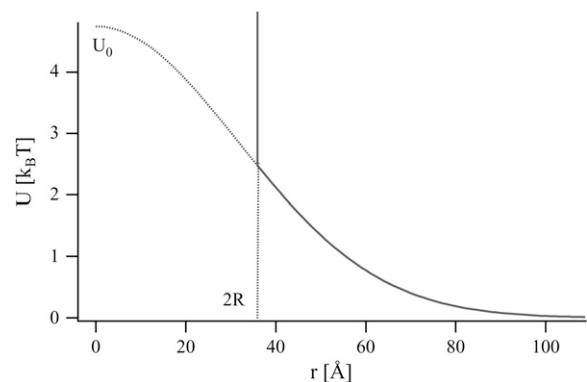
FIGURE 10 The interaction potential used for the fits in Fig. 9, consisting of a hard core and an additional Gaussian repulsion, given by Eq. 5, with parameters U_0 = 4.74 k_B T and \xi = 31.5 \text{ Å} . The contact value U(2R) = 2.41 k_B T .
